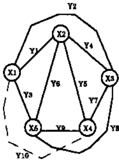
Figure 3: planarity obstructions
