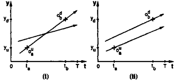
Figure 2: Time space diagrams showing two possible events in the two-car universe, given observations o_a^u and o_b^d (and no other observations). In (i), we have a=b , while in (ii), we have a \neq b .
