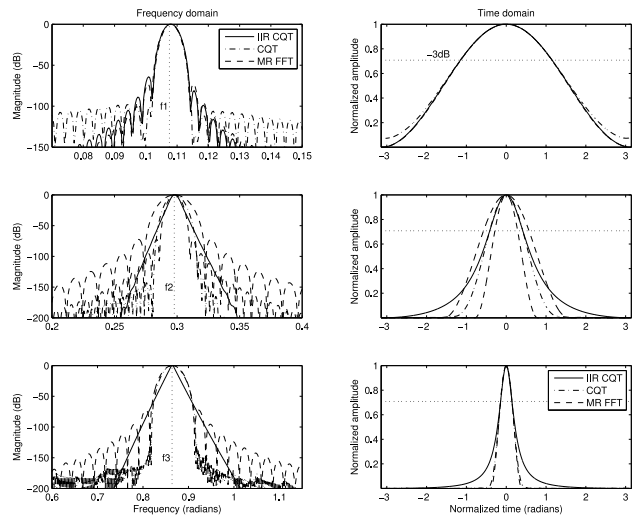
Figure 4. Windows comparison at frequencies f_1 , f_2 and f_3 for the different methods. At f_1 and f_3 the three methods have the same Q, while at f_2 the MR FFT can not achieve the desired Q. For this reason, the two nearest MR FFT windows are considered at f_2 . CQT and MR FFT are computed using a Hamming and Hann windows respectively.
