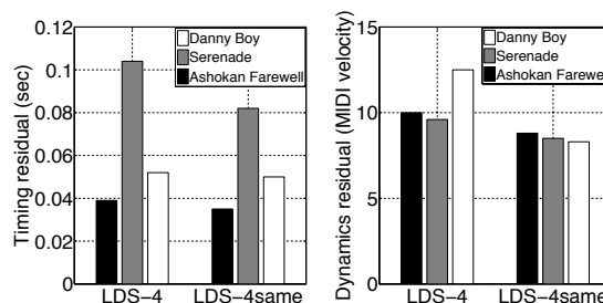
Figure 7. A global view of the performer-specific model.
