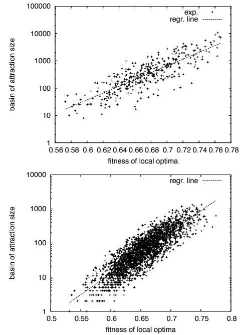
Figure 3: Correlation between the fitness of local optima and their corresponding basin sizes, for two representative instances with N = 18, K = 4 (top) and K = 8 (bottom).
