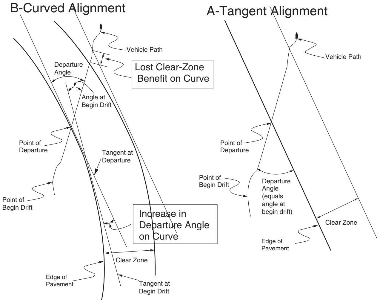
EXHIBIT V-21 Depiction of the Effect of Curvature on the Conditions Resulting from a Vehicle Encroaching on the Roadside
