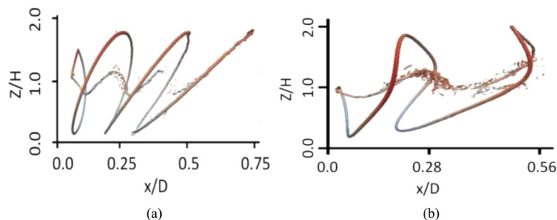
FIG. 14. Tracking the tip-vortex of a single blade WT for (a) LS and (b) HS. Color represents the velocity contours.
