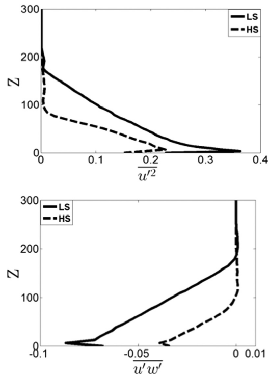
FIG. 5. Time-averaged profile of (a) turbulence intensity of streamwise velocity fluctuation and (b) \overline{u'w'} of stable ABL as low and high stratification.
