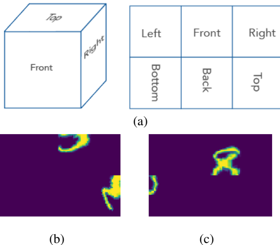
Figure 4. Cube-map projection: (a) schematic illustration of the unwrapping process of the cube surface with a baseball arrangement (Chen et al., 2018) onto a planar surface; (b,c) sample projections of images from the MNIST dataset on the cube surface unwrapped into rectangular images.
