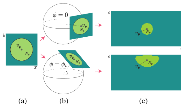
Figure 1. Adaptation of the size and shape of the circular filter defined on a tangent plane (a), which is then projected at different elevations of the spherical surface (b) that, in turn, results in having different projections of the filter area on an equirectangular image (c). Our network is capable of modeling this differences and thus adapting the size and shape of the filter with respect to the elevation in an omnidirectional image.
