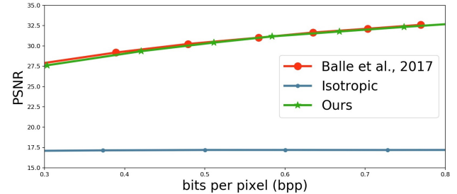
Figure 7. PSNR results of the decompressed images for different filter types with respect to bit per pixel values.
