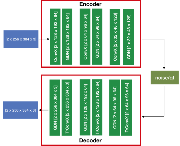
Figure 6. Architecture of compression algorithm. For our experiment we use omnidirectional images projected to the cube surface with a baseball arrangement with size [256 \times 384 \times 3] grouped in batches of size 2. Here, ConvX and TrConvX denote convolutional and transpose convolutional layers with stride 2, where X corresponds to the possible choice of either standard convolutional or proposed geometry-aware graph-based filters; and GDN is a normalization layer which is proposed by (Ballé et al., 2016).
