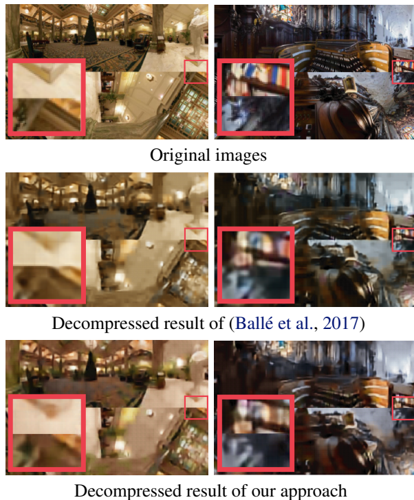
Figure 8. Cube-map projection’s artifacts appear due to the discontinuity between unwrapped face’s borders. In the left corners of original and decompressed images we show zoomed version of the image patch that illustrates the borders of the cube faces. The decompressed results obtained by our anisotropic geometry-aware filters does not smooth border of the faces as our method has access to the information about cube-map geometry, while the result obtained with convolutional filters from (Ballé et al., 2017) smooths these borders. This smoothing can lead to perceptually unpleasant result in various applications (e.g., virtual reality). (best seen in color)
