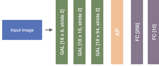
Figure 5. Our classification network consists of three geometry-aware graph-based convolutional layers (GAL) with stride 2. Each of the GAL [X \times Y, \text{stride } 2] convolutional layers contains Y filters with X parameters. The convolutional layers are followed by an average pooling operation AP and two fully-connected layers FC [Z] with Z neurons each.
