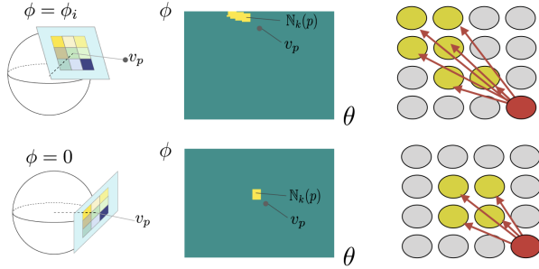
Figure 2. [LEFT] Illustration of the 3 \times 3 GA-filter kernel, defined on the tangent plane. Projection of area s_k forms the neighborhood N_k(p) of the node v_p , where the GA-filter is applied. [MIDDLE] The neighborhood N_k(p) changes depending on the location of v_p and the chosen filter area s_k , for k = 1 (yellow). [RIGHT] The directed connections between the node v_p with the nodes in its neighborhood N_k(p) . (best seen in color)
