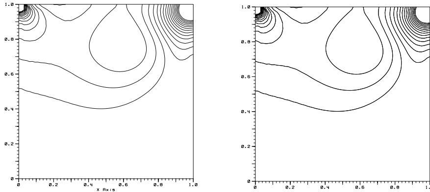
Figure 22: Driven cavity at Re = 100 , 64 \times 64 grid cells: 30 contour lines of the nodal pressure p_v^{(2)} in [-0.4, 0.4] . C = 0.08 (left) and C = 0.008 (right).
