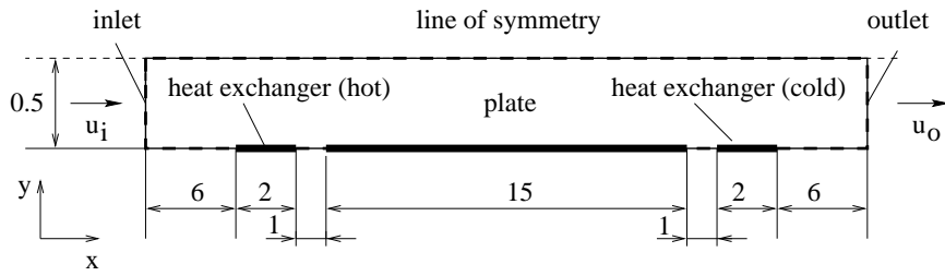
Figure 30: Computational domain (dotted line).
