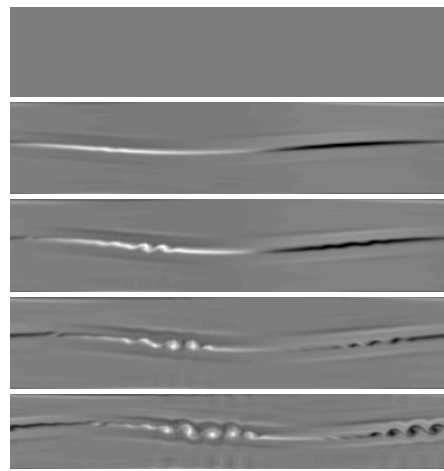
Figure 17: Vorticity at times t=0,6,9,11,14
