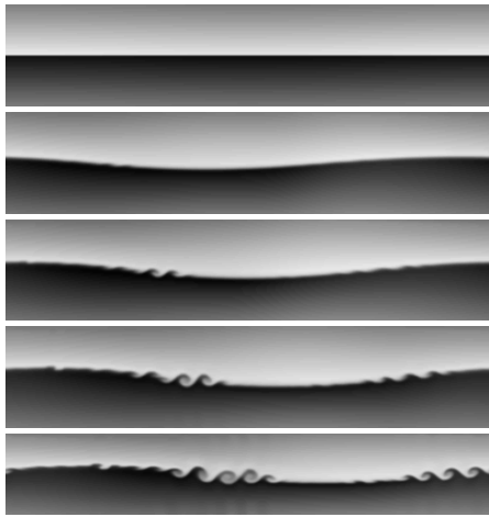
Figure 16: Density at times t=0,6,9,11,14
