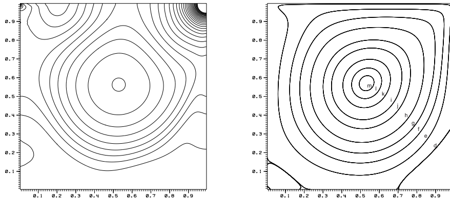
Figure 24: Driven cavity at Re = 1000 , 128 \times 128 grid cells: 30 contour lines of the nodal pressure p_v^{(2)} in [-0.4; 0.4] (left) and streamlines (right). Streamline values and labels from [59].
