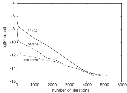
Figure 23: Driven cavity at Re = 1000 : Residual versus number of iterations for 32 \times 32 , 64 \times 64 and 128 \times 128 grid cells computations; coarser grid solutions have been taken as initial data for finer grid solutions.
