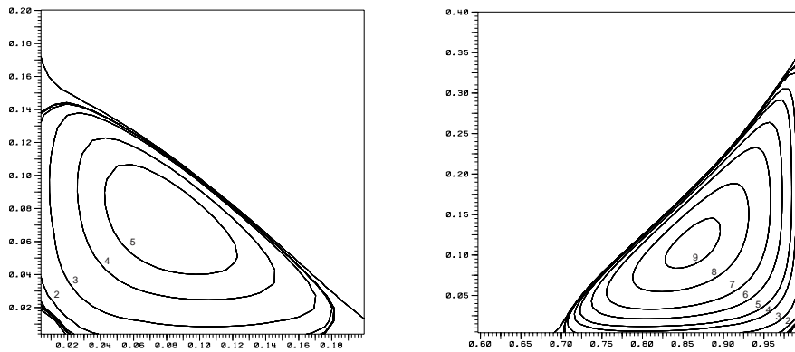
Figure 25: Driven cavity at Re=1000 , 128 \times 128 grid cells: streamlines in the left and right bottom secondary vortices. Values and labels from [59].
