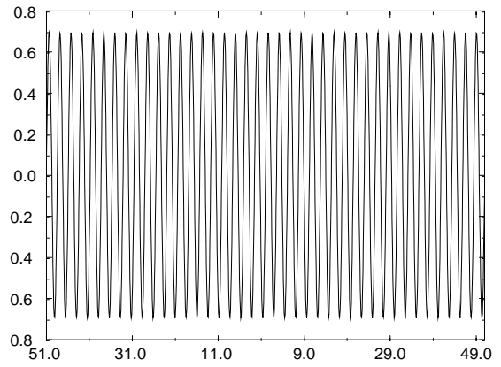
Figure 2: Pressure perturbation
