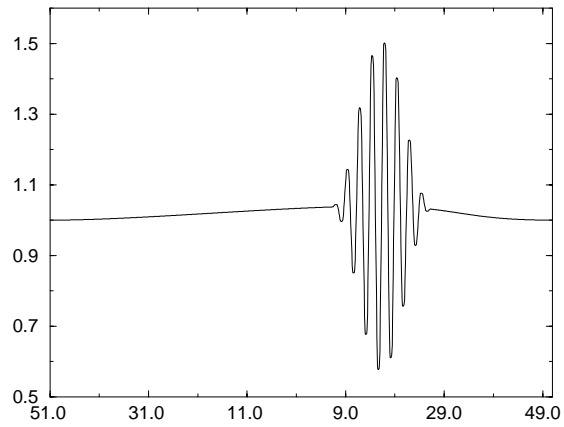
Figure 6: Density profile
