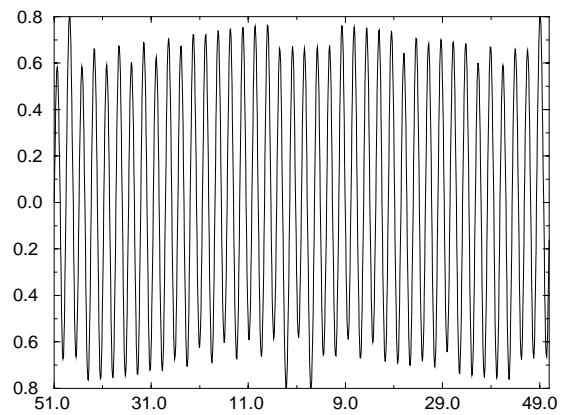
Figure 5: Remaining noise
