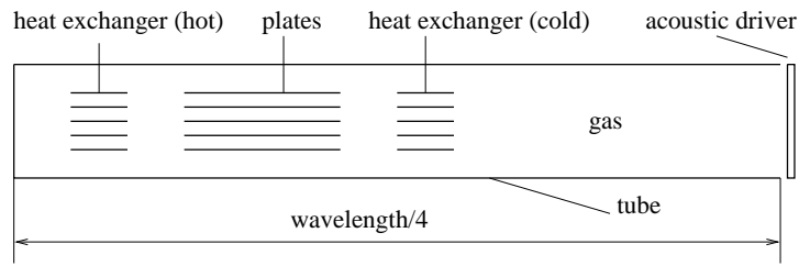
Figure 29: Sketch of a simplified thermo-acoustic refrigerator.
