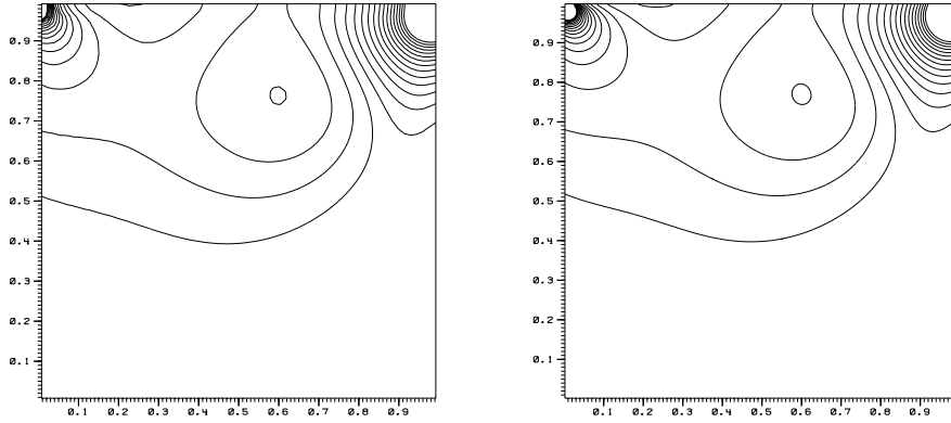
Figure 21: Driven cavity at Re = 100 , C = 0.8 : 30 contour lines of the nodal pressure p_v^{(2)} in [-0.4, 0.4] . 64 \times 64 (left) and 256 \times 256 (right) grid cells.
