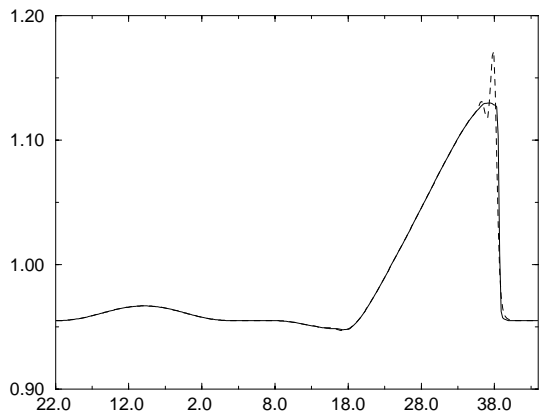
Figure 35: Density distribution at time t = 33 s
