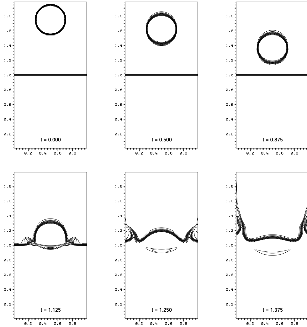
Figure 27: Two-dimensional falling “droplet” at Fr = 1 and density ratio 1000: Contour lines of density in [1, 1000] .
