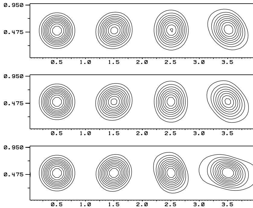
Figure 20: Advection of a vortex at times t = 0.0, 1.0, 2.0, 3.0 : 9 contour lines of the streamfunction in [0.02, 0.18] . Unlimited slopes (top), monotonized central-difference (middle) and Sweby's limiter with k := 1.8 (bottom).
