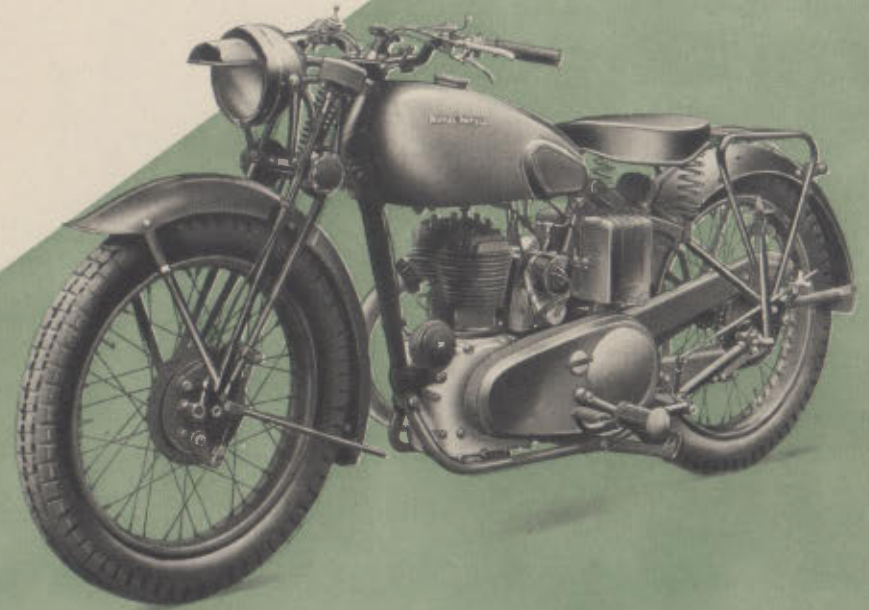
350 c.c. SIDE-VALVE.
