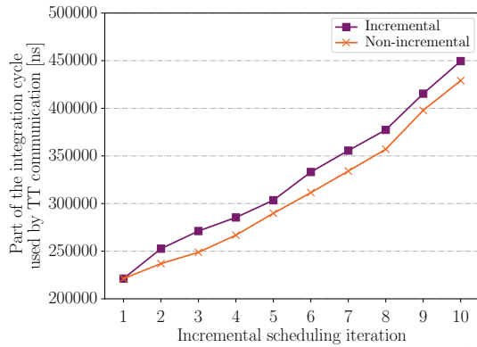
Figure 5: The difference between the incremental and non-incremental scheduling.
