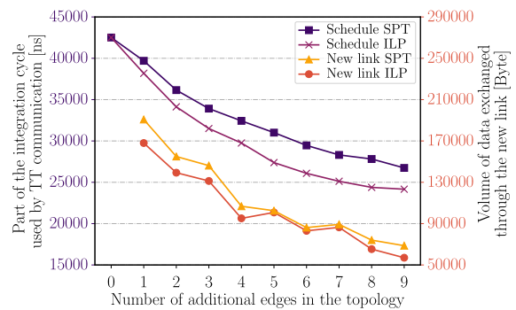
Figure 4: The evaluation of the routing quality.
