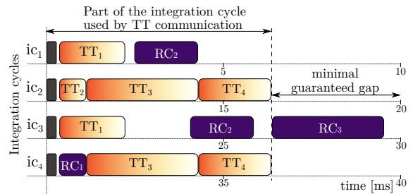
Figure 2: The example of the communication on a link in one cluster cycle.
