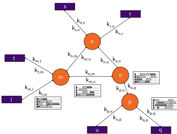
Figure 1: An example of the TTEthernet network topology with the routing and scheduling of message m_1 from node l to node q .
