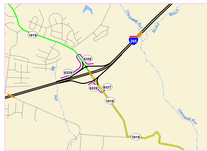
I-265/ KY-1819 INTERSECTION
