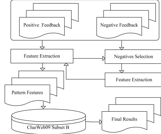
Figure 3. The Stage 2 Architecture
