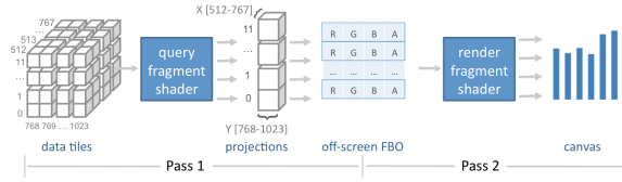
Figure 8: A two-pass approach for parallel data querying and rendering using WebGL fragment shaders.
