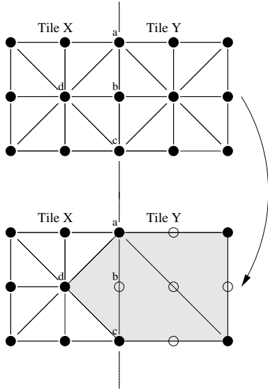
Figure 6: Initially : Both tile X and tile Y are rendered at the same level. After : Tile Y is rendered one level higher. Border morph description : The point b is linearly interpolated between its original value and \frac{(a+c)}{2} . When the morph is completed, tile X is modified by removing the triangles \triangle dab and \triangle dbc and adding the triangle \triangle dac . The shaded area is the area affected by the morphing.
