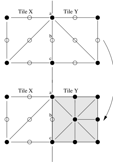
Figure 7: Initially : Both tile X and tile Y are rendered at the same level. After : Tile Y is rendered one level lower. Border morph description : The morphing in tile Y will take place without affecting Tile X. The shaded area is the area affected by the morphing.
