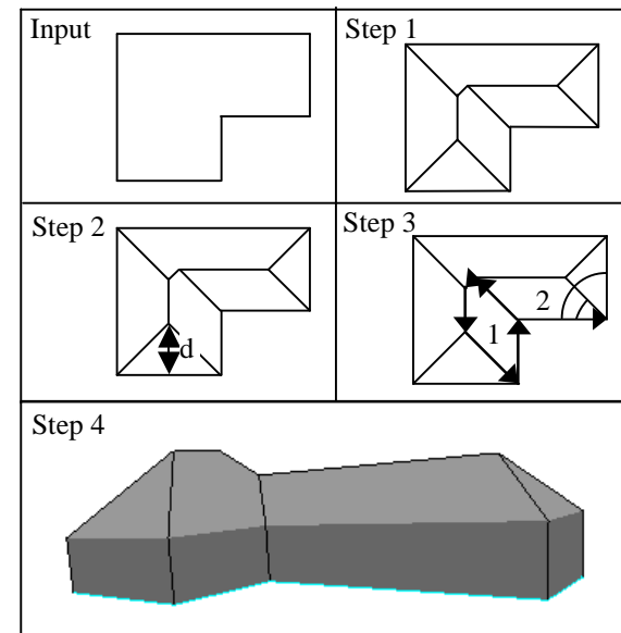
Figure 2: Hip Roof Modelling, [Fel98a]
