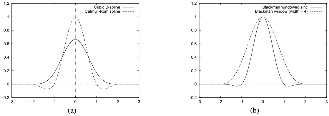
Figure 1: Filter kernels we have used: (a) Cubic B-spline and Catmull-Rom spline; (b) Blackman-windowed sinc depicting also the window itself.
