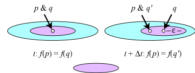
Figure 5: After time \Delta t , a point q' within \varepsilon of q remains in contact with p .
