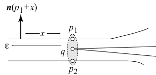
Figure 3: f(p_1) = f(p_2) = q and f((p_1, p_1 + \varepsilon)) = f((p_2, p_2 + \varepsilon)) for some \varepsilon > 0 .
