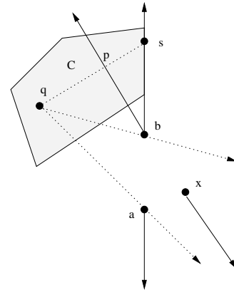
Figure 4: If point s is on chipped line \overline{ab} , there is no point in wedge aqb .
