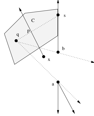
Figure 3: If point s is on chipped line \overline{ab} , there is no point in triangle aqb .
