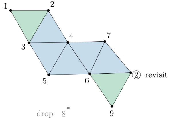
Figure 2: Example of a facet-path.
