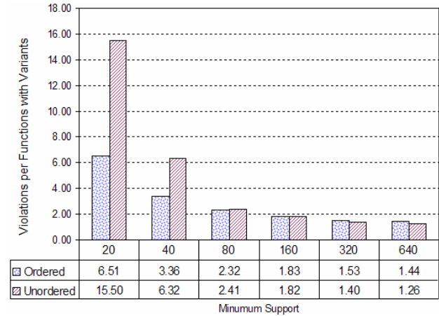
Figure 3. Violations per function with variants showing that sequential-pattern mining outperforms itemset mining for lower support values and performs equally for higher support values.
