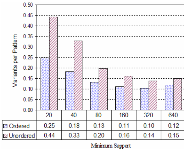
Figure 2. Variants per pattern showing that sequential-pattern mining outperforms itemset mining as the ratio of the number of variants per pattern is always low for ordered patterns.
