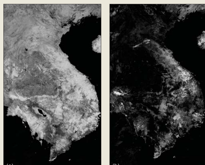
Images of ADEOS-II/GLI 250 m data around the Indochina Peninsula on 7-22 April 2003, showing (a) the NDVI image and (b) the SI image in grayscale. The SI is estimated using the normalization method
