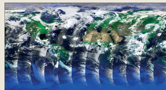
This image is made from FY-1C multi-orbit data on 9 August 2000. It shows how the satellite scans and circles around the Earth. As the influence of the solar zenith angle is not corrected, the edges where orbits meet are obvious. Global image mosaic is the basic form for global environment monitoring and data application
