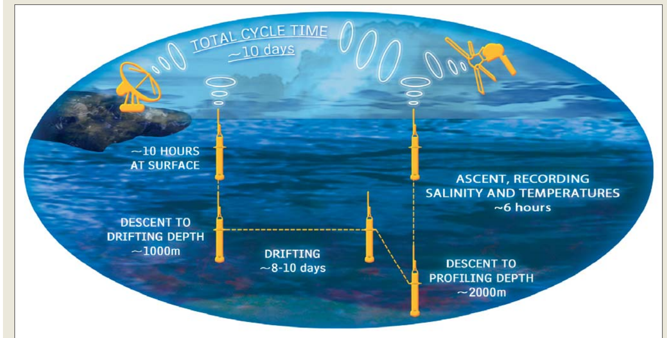
A typical duty cycle for an Argo float
