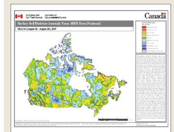
Soil moisture is an indicator of the onset of drought conditions, that could, in turn, adversely effect food production
