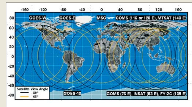
Current and future network of operational geostationary meteorological satellites with active fire detection capabilities
