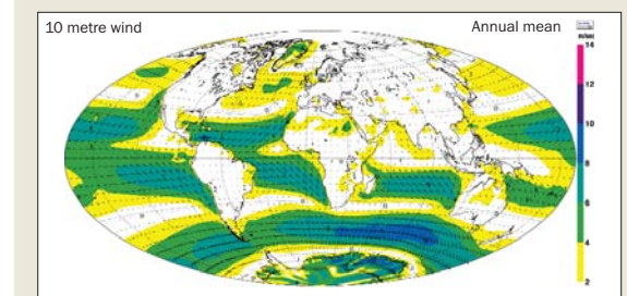
Mean annual near surface wind speed (m/s) and direction 1979–2001
