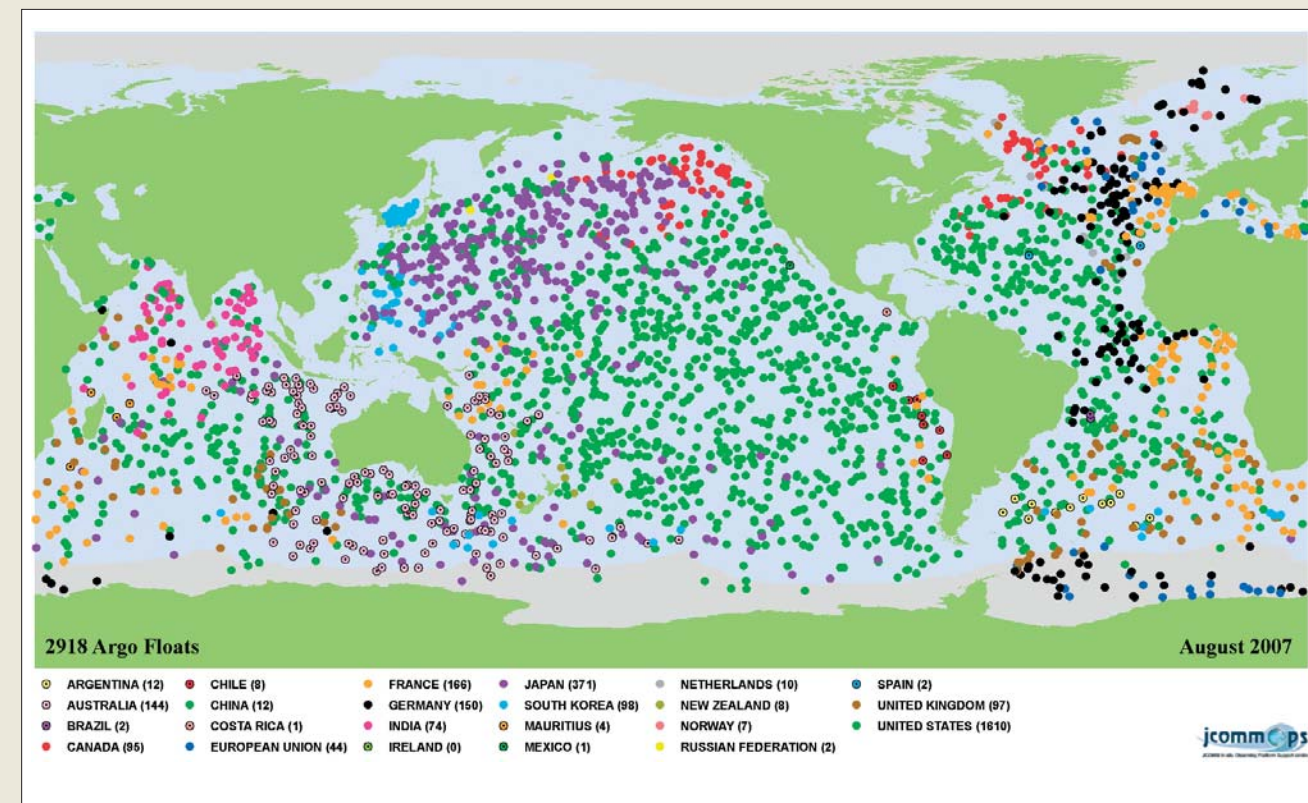
The distribution of floats in the Argo array, August 2007
