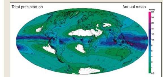
Annual daily mean precipitation (mm/day) 1979–2002
