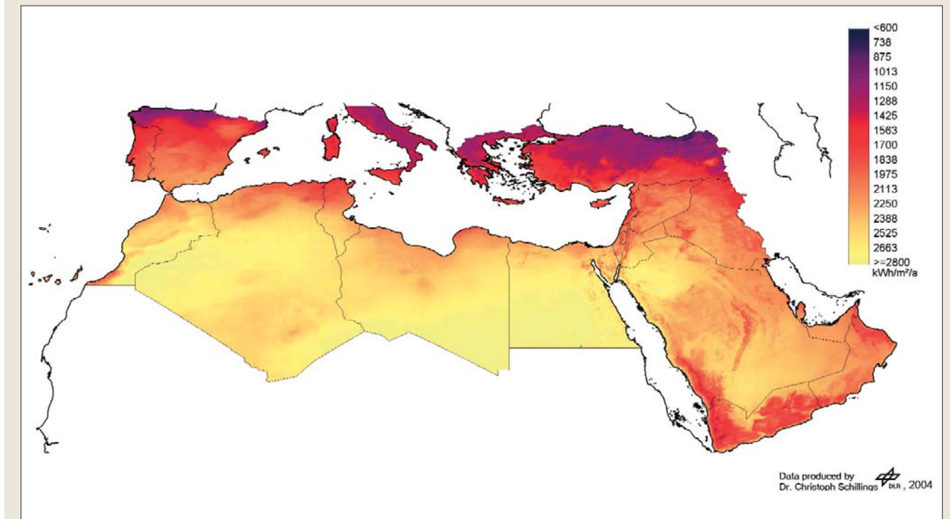
Image showing annual sum of direct normal irradiance for 2004
