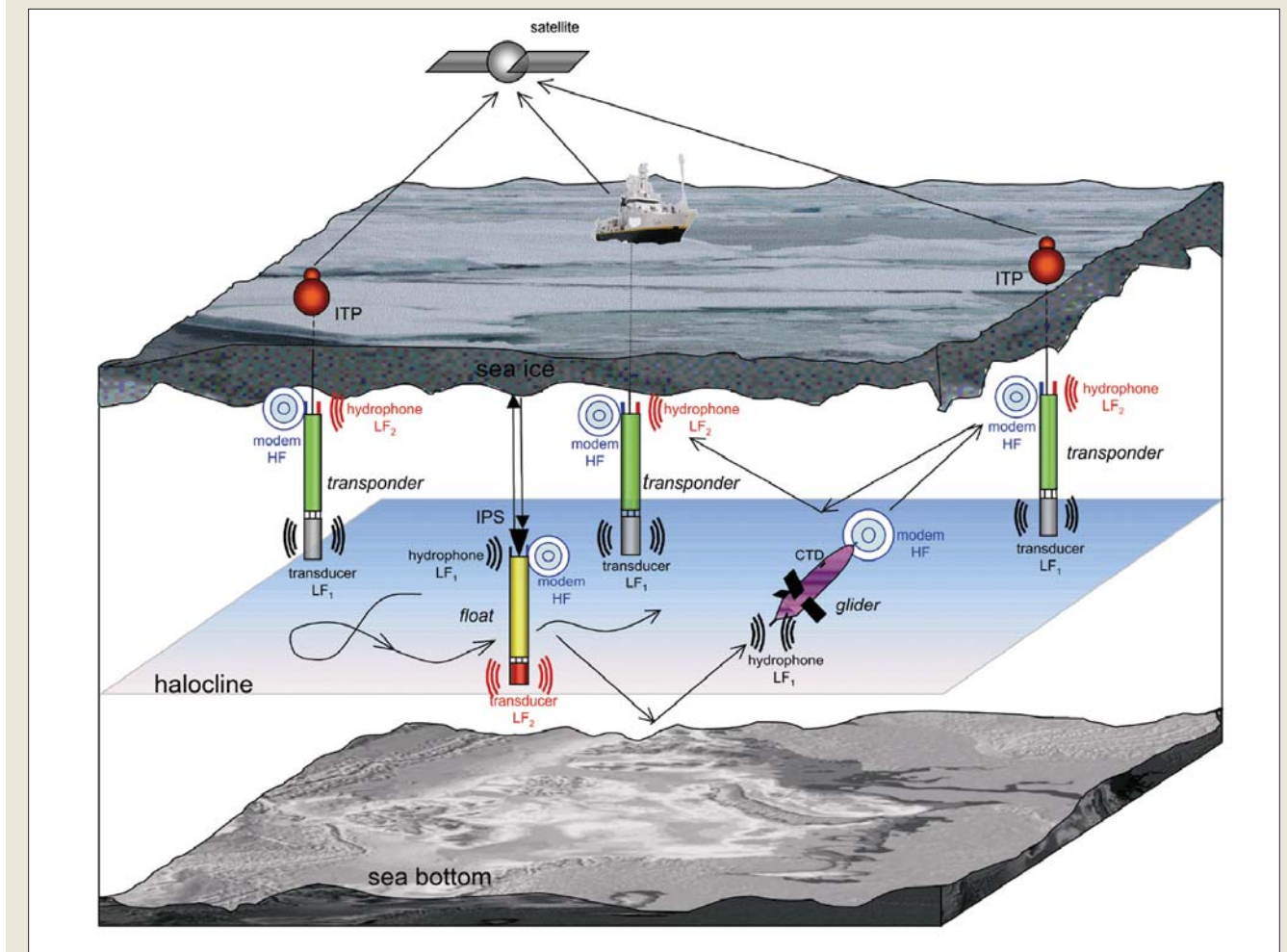
The ocean-observing scheme for the Arctic Ocean currently being implemented by the DAMOCLES Integrated Project of EC-FP6. An extensive system of floats and gliders explore the upper ocean, communicating their data to satellites and receiving measurement-control and navigation information via a net of ice-tethered platforms
