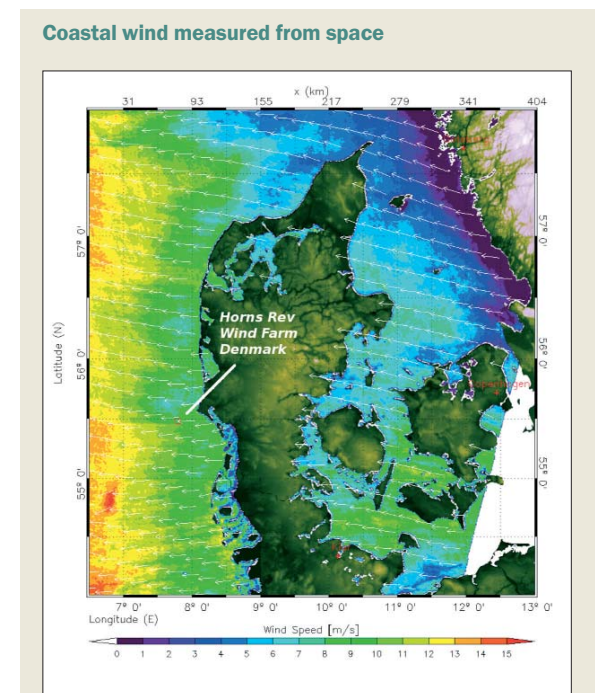
High-resolution wind field (mainly originating from South West) around the Horns Rev wind farm, off the coast of Denmark. Data derived from the ASAR instrument onboard the ENVISAT satellite on the 14 November 2005
