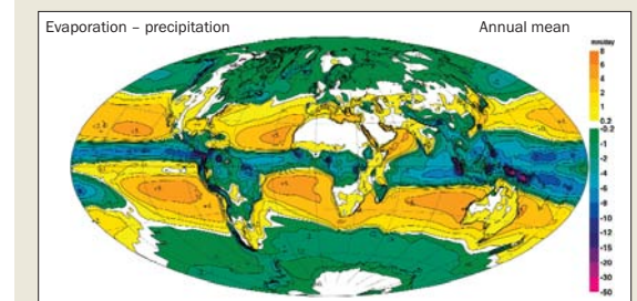
Annual mean evaporation-minus-precipitation (mm/day) 1979–2002
