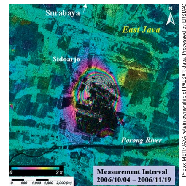
Interferogram derived from a pair of PALSAR data. The circular fringe pattern corresponds to the area affected by land subsidence
