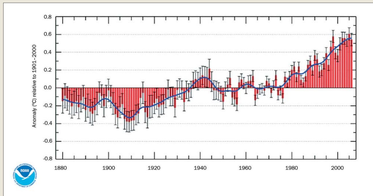
January–December global mean temperature over land and ocean
