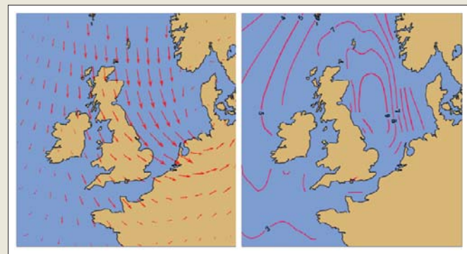
Near-surface wind (maximum speed about 30ms -1 ) and ocean-wave height (metres) from a reanalysis for 00UTC, 1 February 1953, the night of a devastating North-Sea storm.
