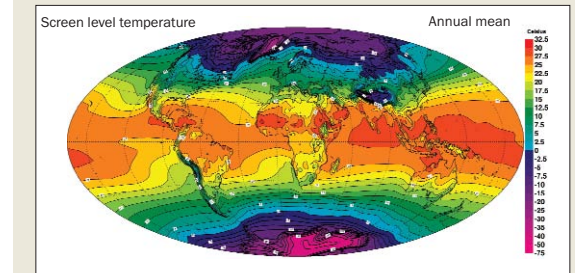
Global mean two-metre temperature 1979–2001
