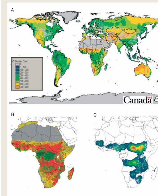
Examples of potential early warning products, including a) global fire danger using the Drought Code (DC) component of the Canadian Forest Fire Weather Index System (Van Wagner 1987); b) DC overlaid by hotspot data (red), and c) spatial fire threat as assessed by DC and hotspot density
