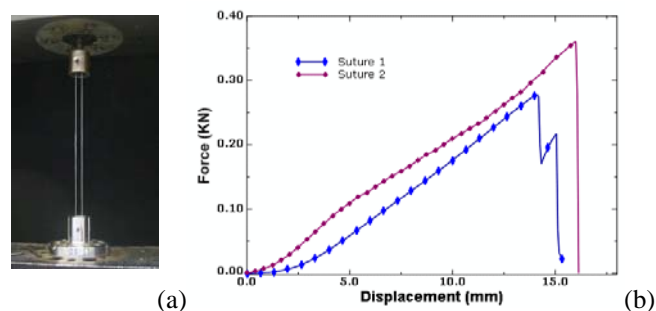
Fig. 3. Experimental setup of the test (a); and load-displacement result of two rigidly clamped looped sutures.
