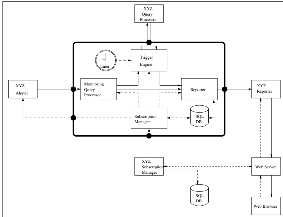
Figure 3: Architecture for the subscription system
