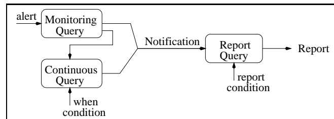
Figure 1: Main Components of a Subscription
