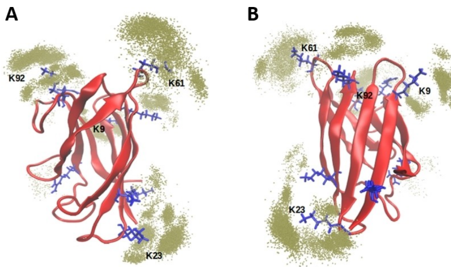
Figure 4. Structural representation of the localization of CLR01 molecules. The \text{SOD1}_{\text{bar}} is represented in red, lysine and arginine residues are highlighted in blue licorice and the green dots depict the positions of the phosphorous atoms of the tweezers within 4 Å of any heavy atom of each lysine residue. A and B are different views of the structure, rotated 180° around the central axis of the barrel.
