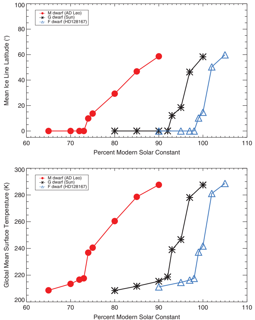
FIG. 8. Mean ice line latitude (top) and global mean surface temperature (bottom) as a function of percent of modern solar constant after a 40-year GCM run for an aqua planet orbiting the Sun (asterisks), M-dwarf star AD Leo (circles), and F-dwarf star HD128167 (triangles) at equivalent flux distances. The slope of each line is a measurement of the climate sensitivity of the planet to changes in stellar flux. The shallower slope of the M-dwarf planet indicates a smaller change in surface temperature and ice extent for a given change in instellation than on the planets orbiting stars with greater visible and near-UV output.
