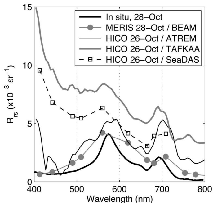
Figure 9. Fall 2011 study: Ground truth optical measurements acquired along the periphery of a red tide patch on 28 October 2011 (location shown in Figure 8b). The in situ R_{rs} spectrum was acquired 59 minutes after the MERIS image. HICO spectra are 3 \times 3 pixel means from the location shown in Figure 7c (zoom panel).
