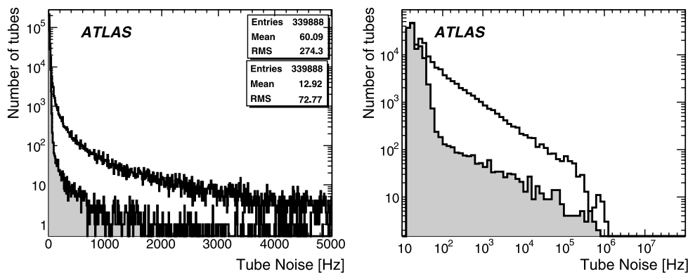
Fig. 13 Distribution of the drift tube noise rate with ( shadowed histogram, bottom statistical box ) and without ( empty histogram, top statistical box ) the ADC cut described in the text. In the right plot the logarithmic scale allows observation of the very few noisy tubes.
