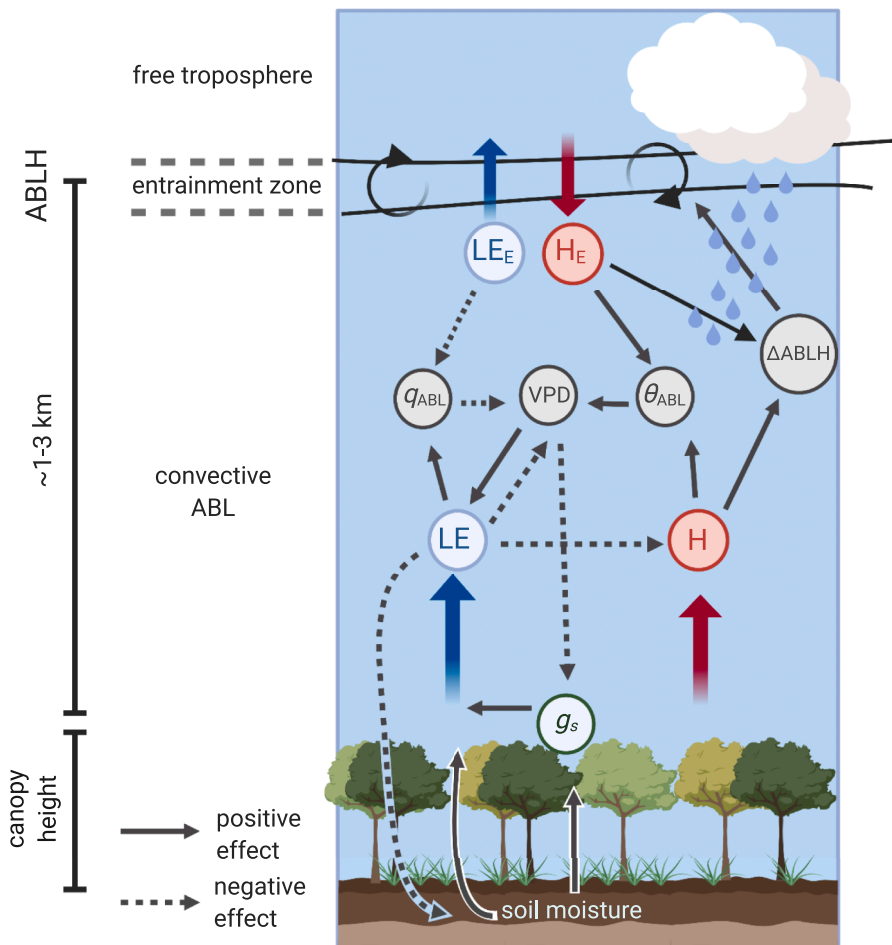
Fig. 4. Daytime interactions and feedbacks between surface sensible ( H ) and latent heat ( LE ) fluxes, entrainment fluxes ( LE_E , H_E ), atmospheric boundary layer growth rate ( \Delta ABLH ), land surface (e.g., soil moisture) and vegetation conditions (e.g., stomatal conductance [ g_s ]), and state of the atmospheric boundary layer (i.e., vapor pressure deficit [ VPD ], mixed-layer potential temperature [ \theta_{ABL} ], and mixed-layer specific humidity [ q_{ABL} ]). The ABL top separates the convective ABL from the free troposphere. This separation zone is defined as the atmospheric boundary layer height (ABLH). Note that ABLH is not constant in time, and that horizontal advection (not shown) will also impact ABL quantities.
