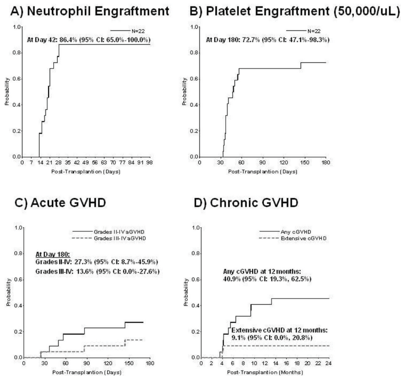
Figure 1. ENGRAFTMENT
