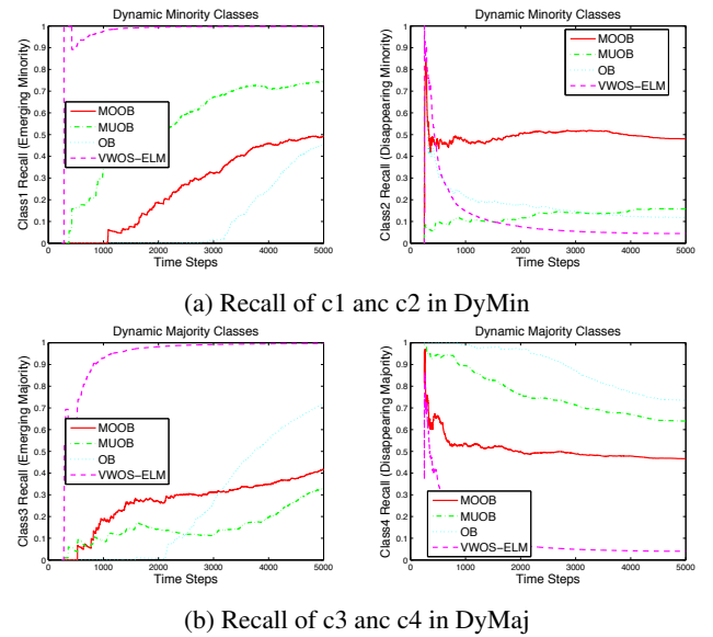
Figure 2: Prequential recall curves of dynamic classes in DyMin and DyMaj.
