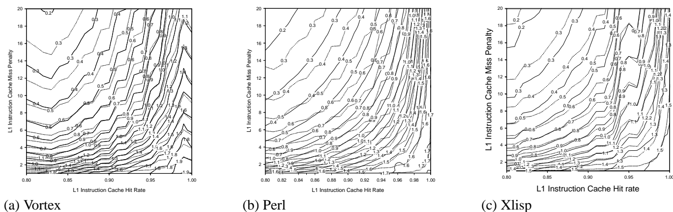
Figure 10: Multi-value correlation between SimpleScalar and the Statistical Simulator for L1 I-cache hit rate vs. L1 I-cache miss penalty.
