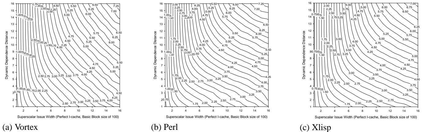
Figure 24: Super-scalar issue width versus dynamic instruction distance assuming a perfect I-cache and basic block size of 100 instructions
