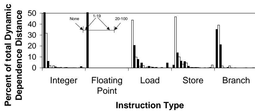
(c) Xlisp
