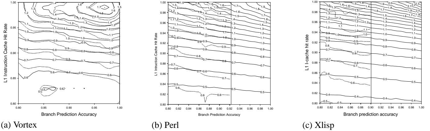
Figure 9: Multi-value correlation between SimpleScalar and the Statistical Simulator for L1 I-cache hit rate and branch prediction accuracy.
