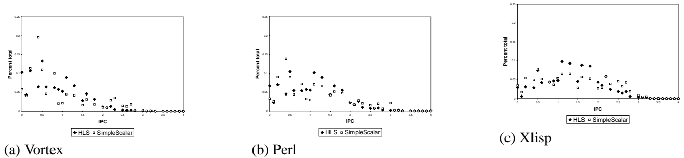
Figure 21: Histogram of IPC samples from HLS and SimpleScalar
