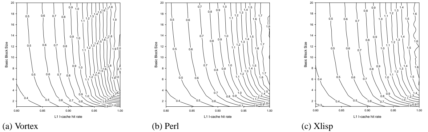
Figure 13: L1 I-cache hit rate versus basic block size
