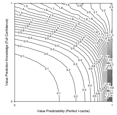
(c) Xlisp
