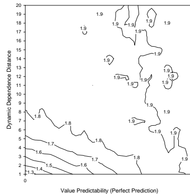
(c) Xlisp
