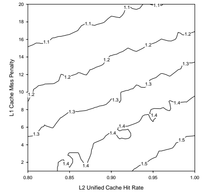
(c) Xlisp
