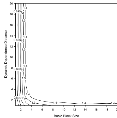
(c) Xlisp
