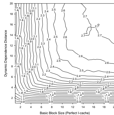
(c) Xlisp
