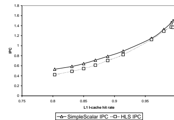
(c) Xlisp
