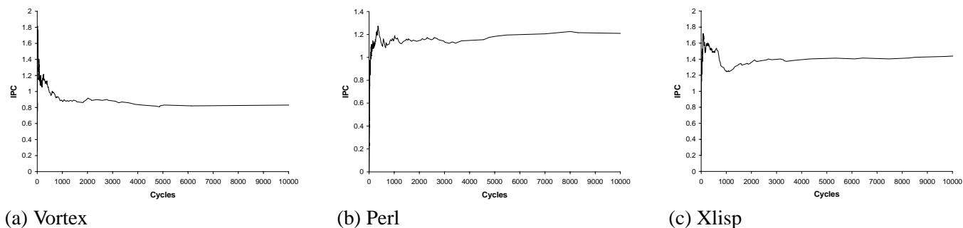
Figure 4: Simulation IPC convergence time (cycles)
