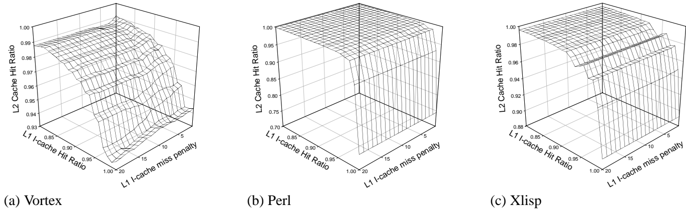
Figure 22: Variation in Unified L2 cache hit rate as L1 I-cache hit rate varies compared to L1 I-cache miss penalty
