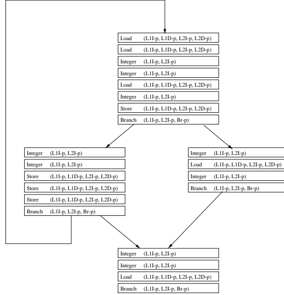
Figure 5: Simulated code example
