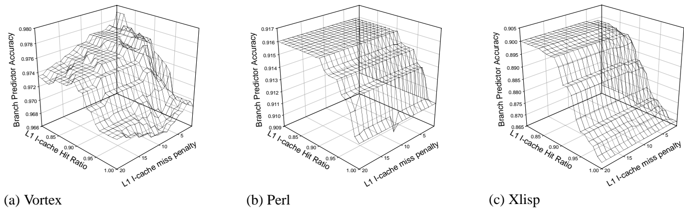
Figure 23: Variation in branch predictor accuracy as L1 I-cache hit rate varies compared to L1 I-cache miss penalty
