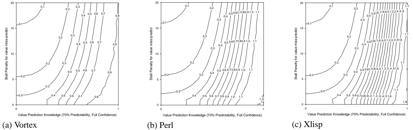
Figure 18: Value prediction knowledge versus mis-speculation penalty
