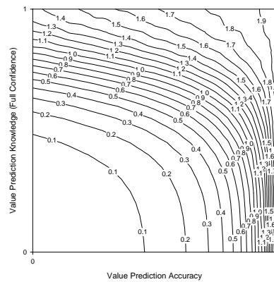
(c) Xlisp
