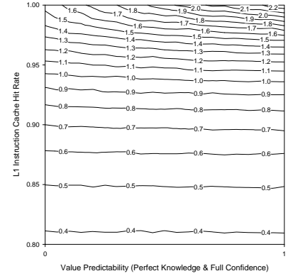
(c) Xlisp
