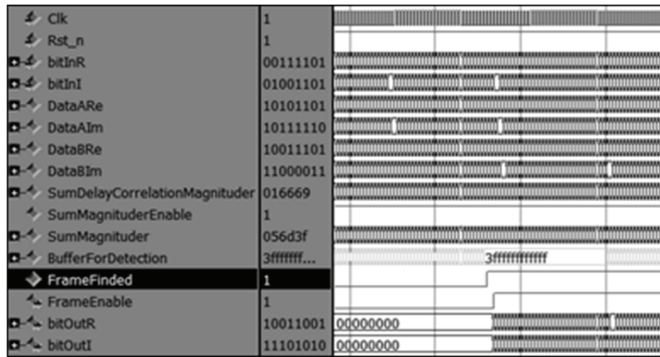
Fig. 13. ModelSim simulation result of coarse synchronization module.
