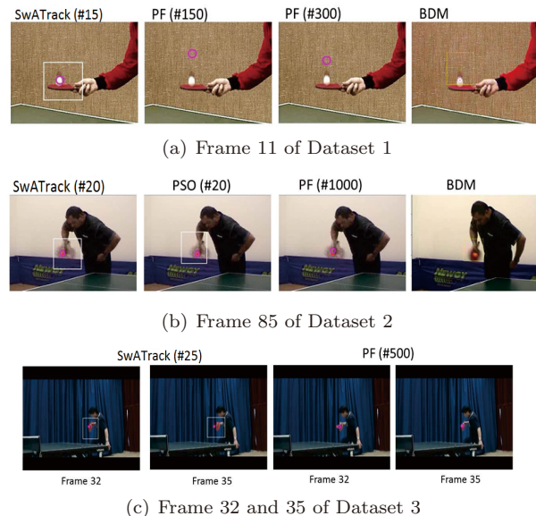
Figure 1. A comparison between our proposed method - SwATrack, PF, PSO and BDM on three publicly available datasets.
