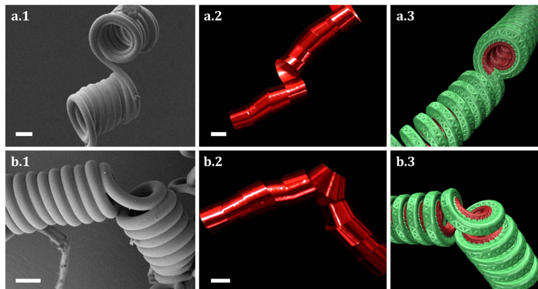
Figure 5. Final configuration for helices connected by antisymmetric and symmetric perversions.
