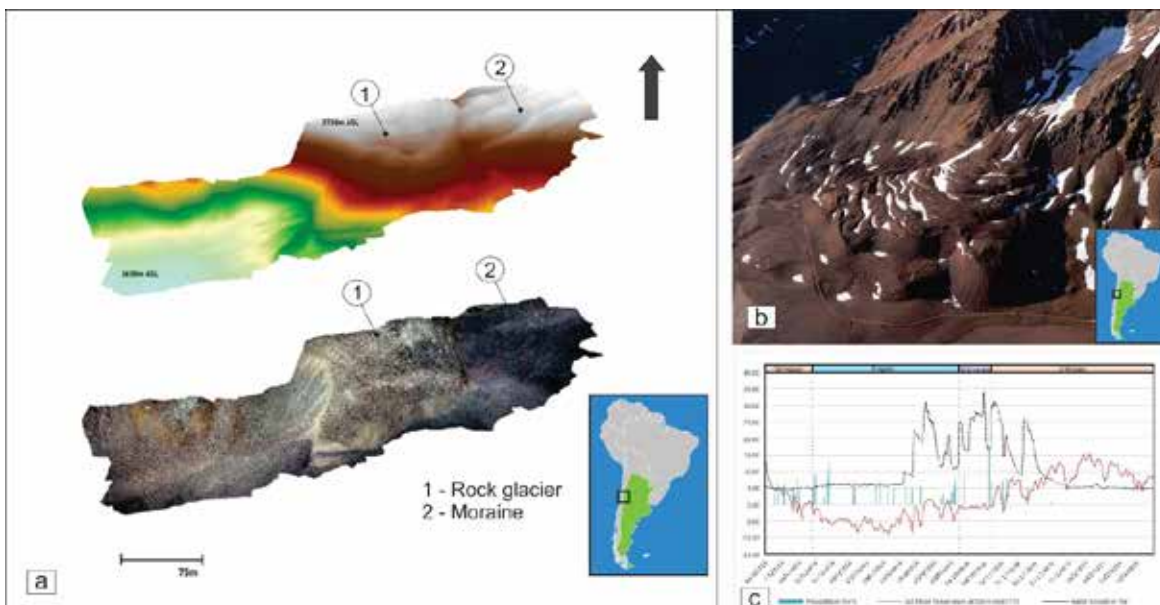
Figure 1: a) Analyzed geoforms located at 32°59'44.71"S; 70° 2'53.70"W within “Monos de Agua” catchment, Aconcagua Basin, Chile. b) Monitored “Candidato” rock glacier located at 31°53'S and 70°11'W, Central Andes, Argentina. c) Soil temperature and volumetric water content during 2018 at 50 cm depth in 4030 m ASL.
