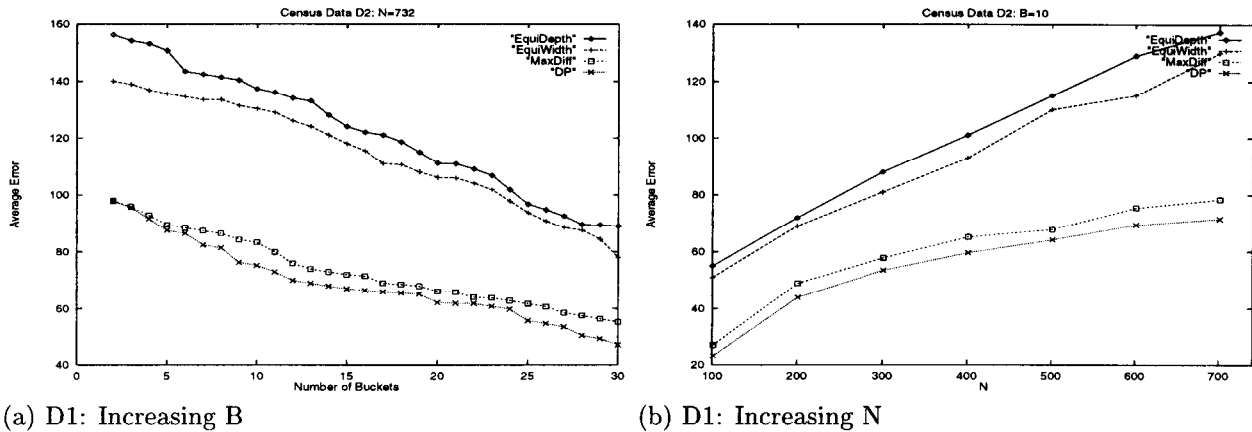
Figure 10: DP, EquiWidth, EquiDepth, MaxDiff for D1
