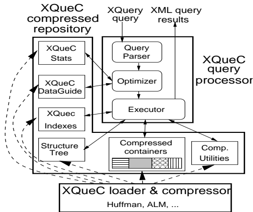
Figure 1: Architecture of the XQueC prototype.
