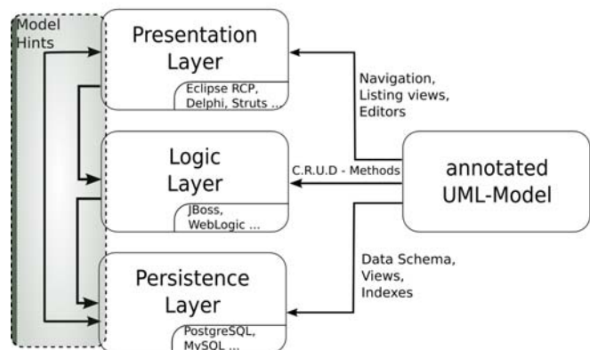
Figure 1: GignoMDA Approach
