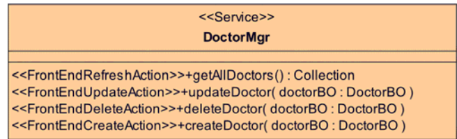
Figure 5: Sample Service
