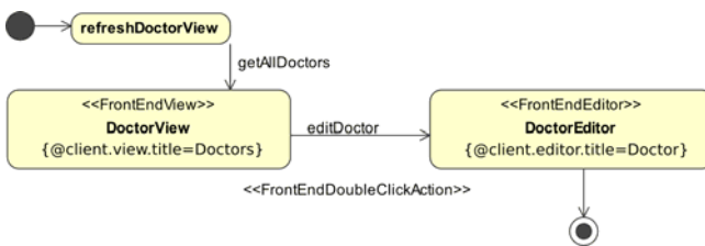
Figure 4: Activity Diagram
