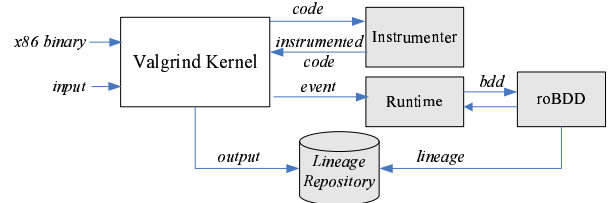
Figure 5: Slicing Infrastructure.
