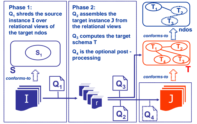
Figure 5: The architecture of the two-phase query generation.
