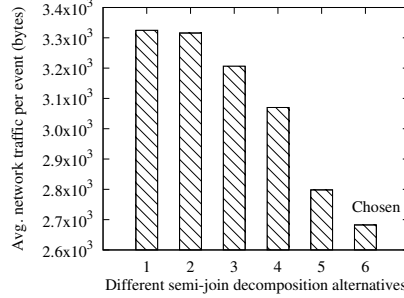
Figure 13: Network traffic; multi-way join mix, general schema.
