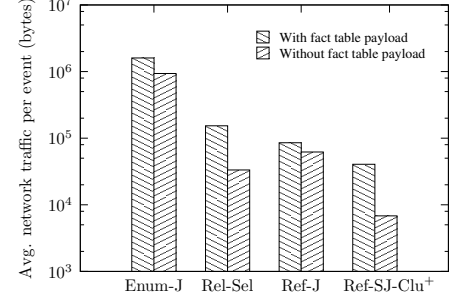
Figure 14: Network traffic; multi-way join mix, star schema.
