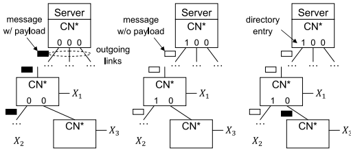
Figure 4: Payload dissemination using CN*.
