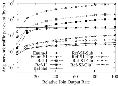
Figure 9: Network traffic; increasing relative join output rate (RJOR).
