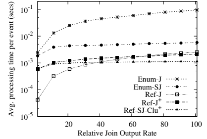
Figure 8: Processing time; increasing relative join output rate (RJOR).
