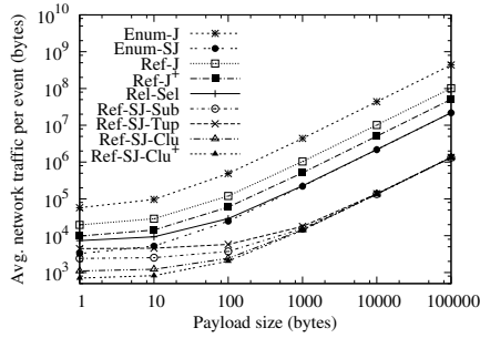
Figure 18: Network traffic; increasing payload size.
