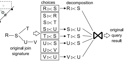
Figure 3: Multi-way decomposition.
