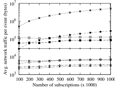
Figure 6: Network traffic; increasing number of subscriptions.
