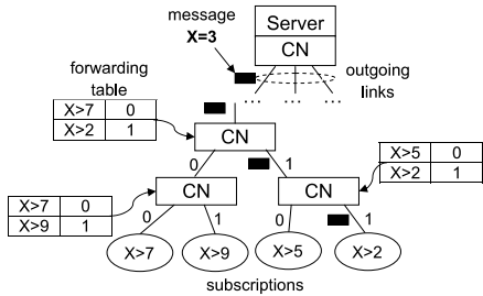
Figure 15: Using a content-based network for publish/subscribe.
