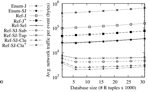
Figure 7: Network traffic; increasing database size.
