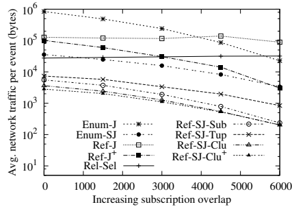
Figure 19: Network traffic; increasing subscription overlap.
