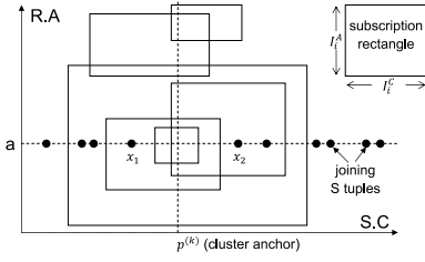
Figure 1: Processing Enum-SJ using SSI for cluster \mathcal{X}^{(k)} .
