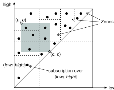
Figure 16: Using a content-addressable network for publish/subscribe.
