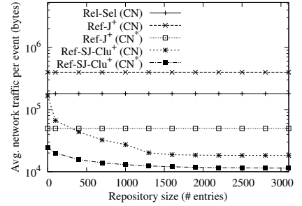
Figure 11: Network traffic; increasing repository size.
