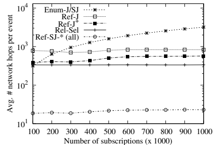
Figure 17: Network hops; increasing number of subscriptions.
