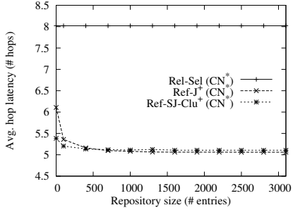
Figure 12: Hop latency; increasing repository size.
