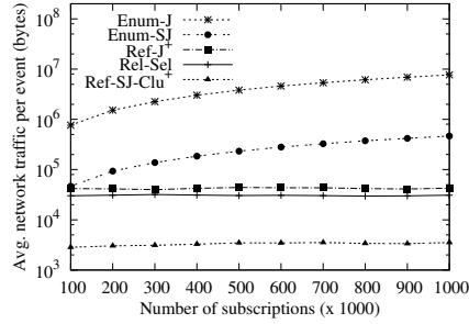
Figure 10: Network traffic; real event workload.
