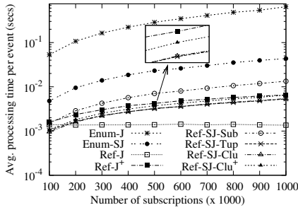
Figure 5: Processing time; increasing number of subscriptions.
