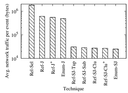
Figure 20: Network traffic; considering last hop.
