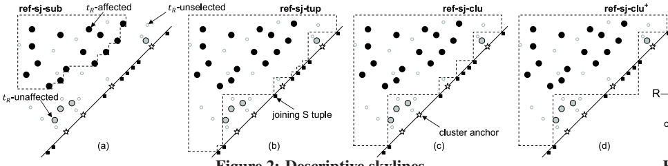
Figure 2: Descriptive skylines.
