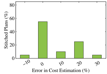
Figure 12: Cost estimation for Cust3
