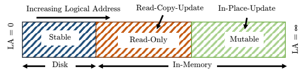
Figure 3: Logical address space in HybridLog.
