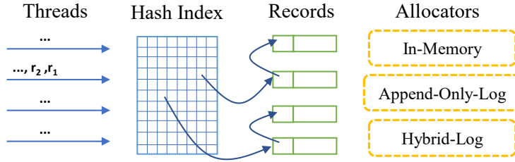
Figure 2: Overall FASTER architecture.
