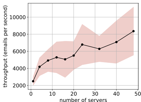
Figure 8: Peak throughput vs number of MillWheel servers using the simple streaming implementation from Figure 5. Standard deviations are shaded red.
