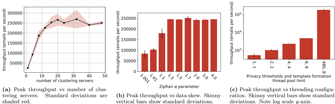
Figure 7: Crusher evaluation.
