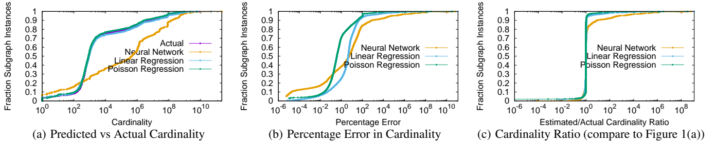
Figure 8: Cross-validation performance.
