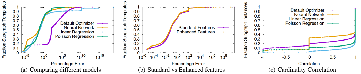
Figure 6: Cardinality model training results.
