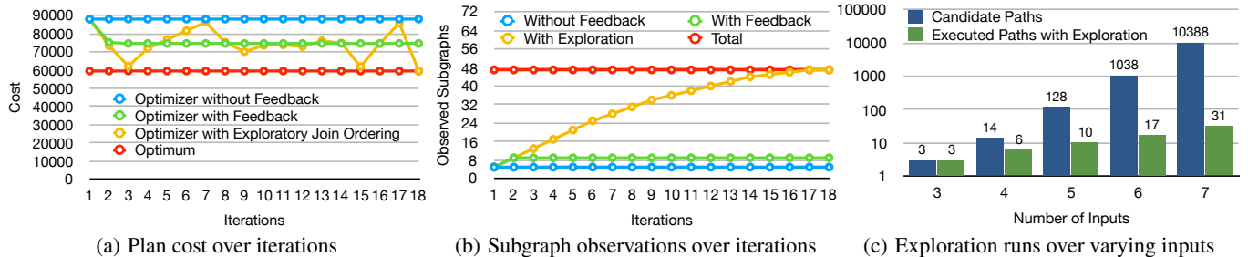
Figure 13: Evaluating the effectiveness of exploratory join ordering.
