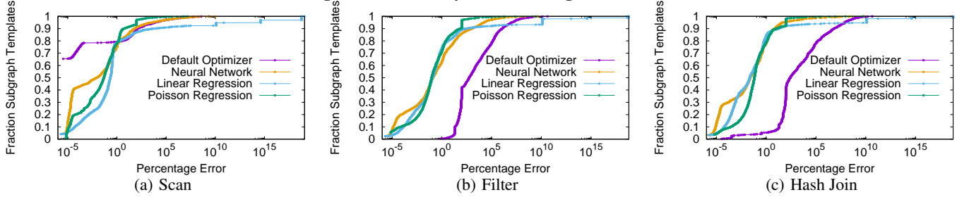
Figure 7: Operator-wise cardinality model training error.
