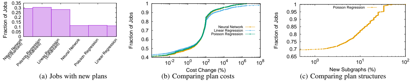
Figure 11: Plan evaluation with the learned cardinality models over production workloads.
