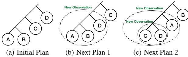
Figure 4: Candidate exploration plans for a recurring query A \bowtie B \bowtie C \bowtie D .
