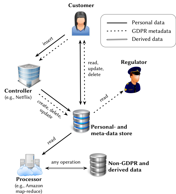
Figure 1: GDPR defines four roles and distinguishes between three types of data. The arrows indicate read-only access, while the arrows into it modify it. (1) The controller can collect, store, delete and update any personal- and GDPR-metadata, (2) A customer can read, update, or delete any personal data and GDPR-metadata that concerns them, (3) A processor reads personal data and produces derived data, and (4) Regulators access GDPR metadata to investigate customer complaints.
