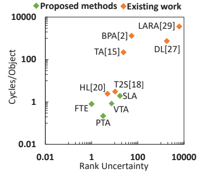
Figure 2: Cycles/Object vs Rank Uncertainty.
