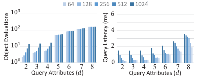
Figure 11: Block size vs latency-object evaluations.
