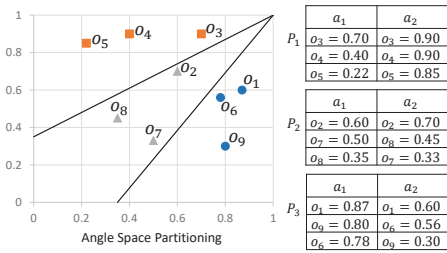
Figure 6: ASP on objects from Fig 3.
