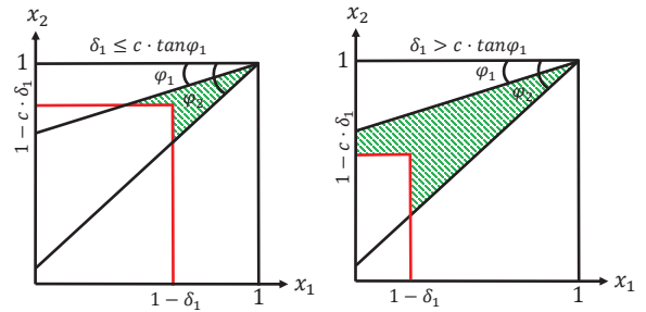
Figure 7: Processed areas for varying \delta_i using ASP.
