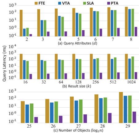
Figure 15: Latency using SIMD instructions.
