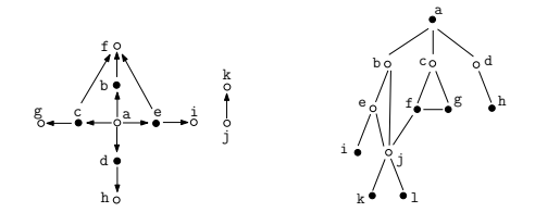
Figure 1: Illustration of the representative MVA problems (0-vertices in white and 1-vertices in black)
