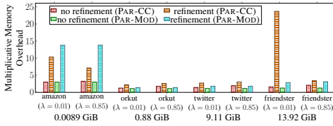
Figure 8: Multiplicative memory overhead, over the size of the input graph, of PAR-CC and PAR-MOD, on amazon, orkut, twitter, and friendster, with \lambda = 0.01, 0.85 . The labels below denote the size of the input graph.
