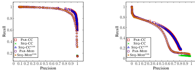
Figure 9: Average precision and recall compared to ground truth communities on amazon (left) and orkut (right) of the clusters obtained from PAR-CC and PAR-MOD, compared to SEQ-CC and SEQ-MOD, using varying resolutions.
