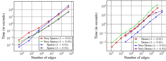
Figure 6: Scalability of PAR-CC over rMAT graphs of varying sizes.
