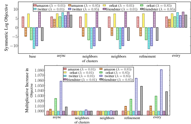
Figure 3: CC objective for PAR-CC on a symmetric log scale 5 (top) and multiplicative increase in the modularity for PAR-MOD over no optimizations (bottom), of each optimization and every optimization. Objectives were obtained on amazon, orkut, twitter, and friendster, with \lambda = 0.01, 0.85 .
