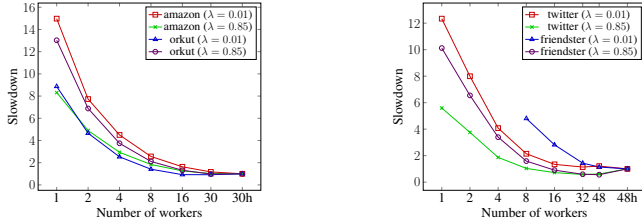
Figure 7: Scalability of PAR-CC over different numbers of threads, on amazon, orkut, twitter, and friendster, with \lambda = 0.01, 0.85 . 30h and 48h indicate 30 and 48 cores respectively, with two-way hyper-threading.
